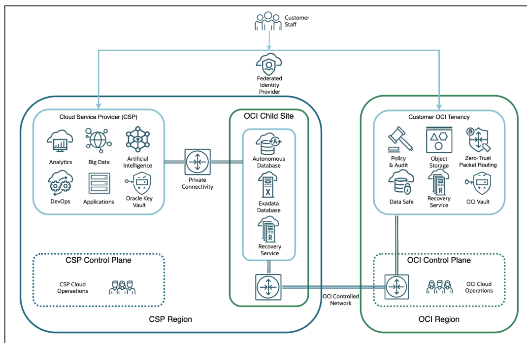
Figure 5: Multicloud Architecture
